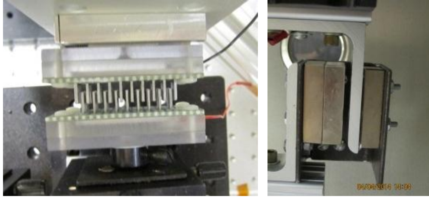
Figure 3. Electrostatic Fins Calibration System and Magnetic Damper
