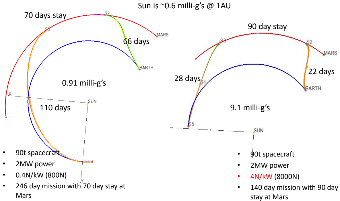
Figure 24. 2MW NEP Roundtrip Mission to Mars with 0.4N/kW e and 4.0 N/kW e thrust to power
