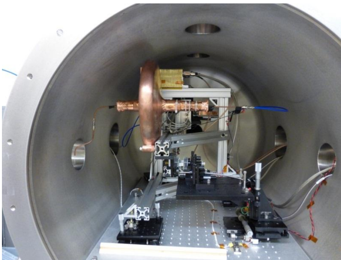
Figure 9. Cannae Test Article on Torsion Pendulum (thrust to the left, a.k.a. forward orientation)
